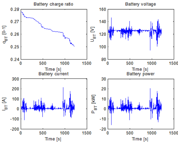
Figure 6. Battery Performance without the supercapacitor module in a pure electric vehicle model.
